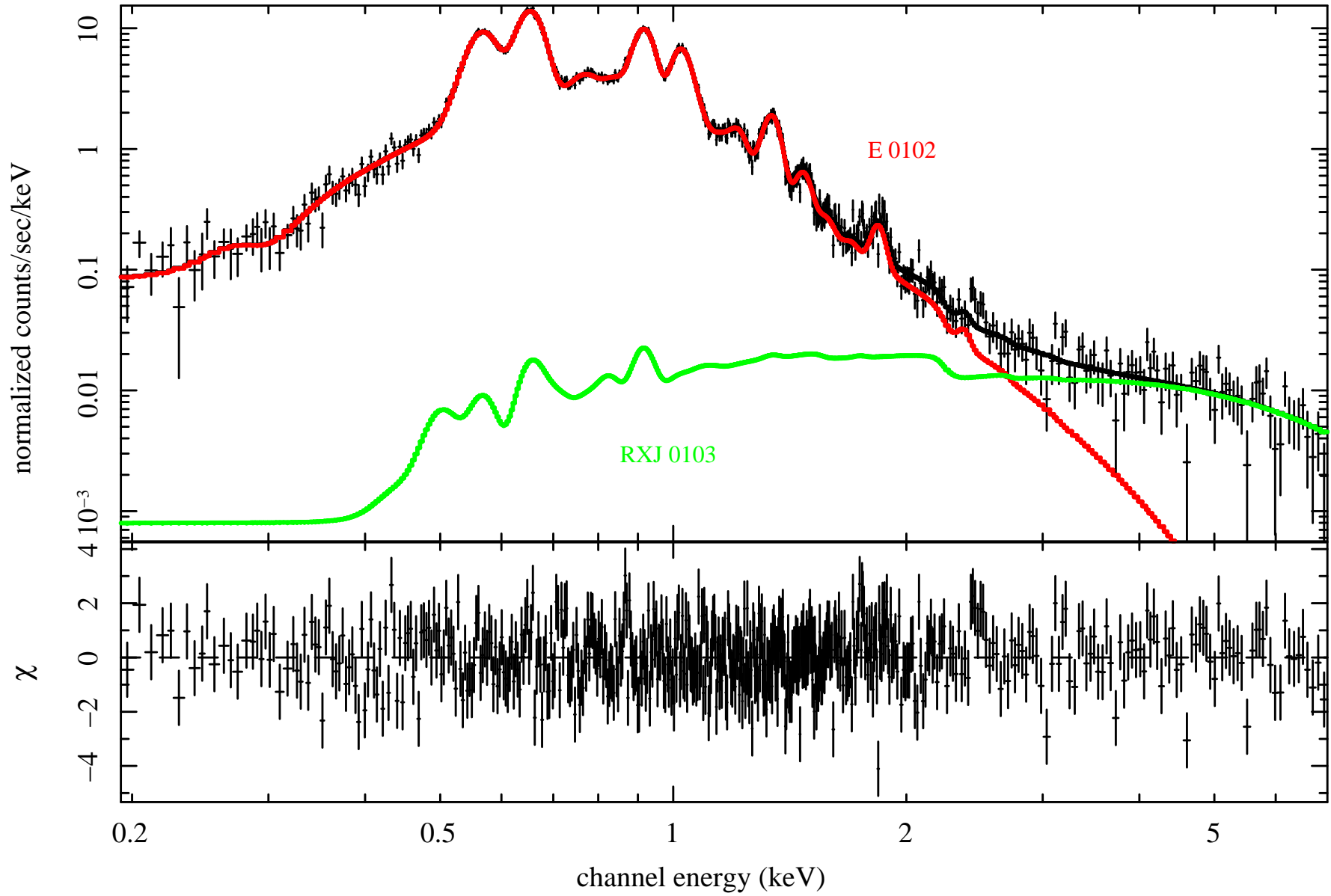
E0102 + RXJ0103 model – XIS1, 2005–08–31
