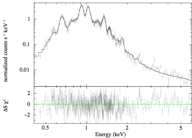
1 E0102-72.3 - XIS3, 20071202
