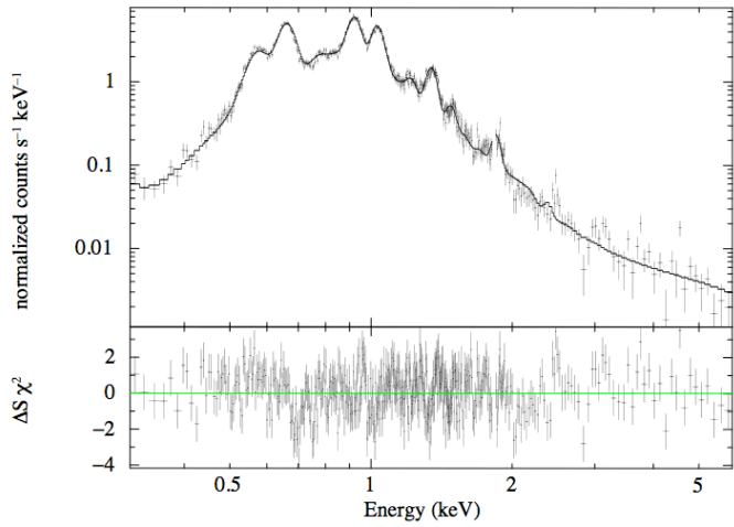
1 E0102-72.3 - XIS1, 20071202
