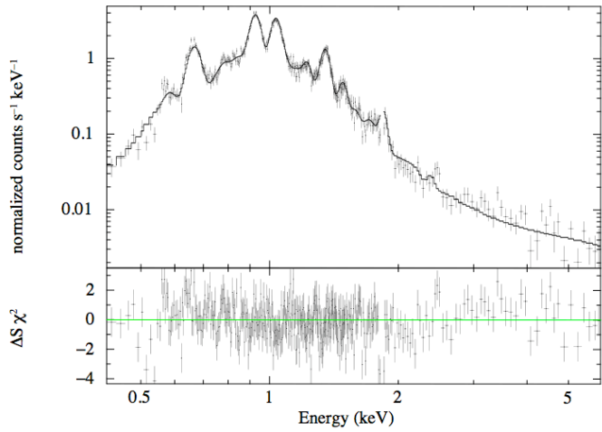
1 E0102-72.3 - XIS0, 20071202
