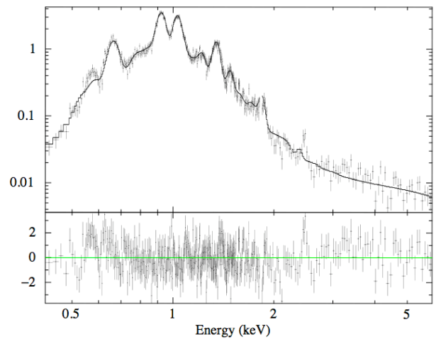
1 E0102-72.3 - XIS3, 20080215
