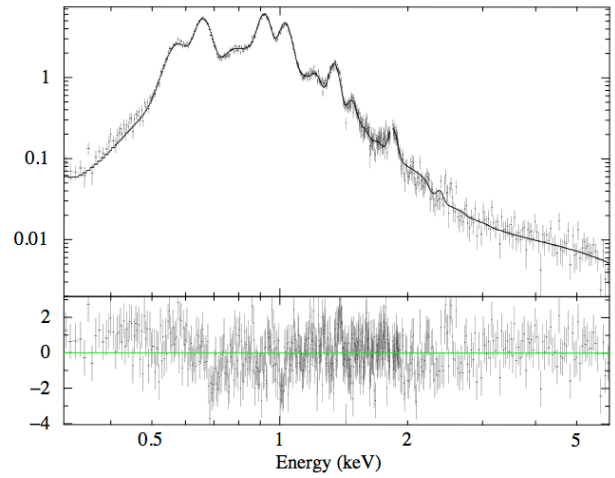
1 E0102-72.3 - XIS1, 20080215
