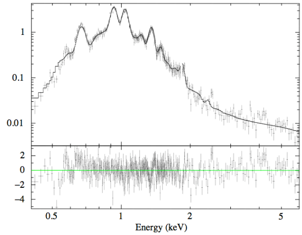
1 E0102-72.3 - XIS0, 20080215
