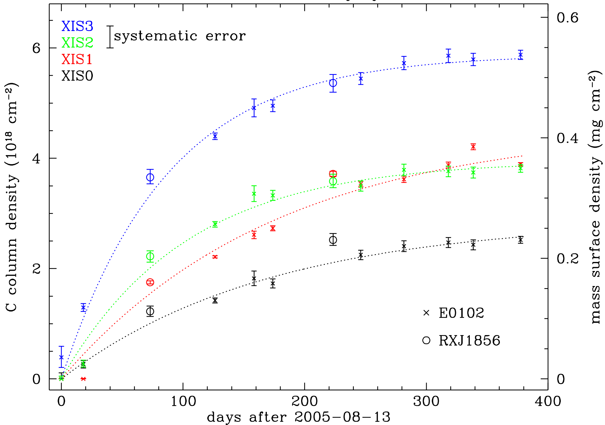
Suzaku/XIS contamination history, N_c/N_0 = 6 assumed, rev0.7
