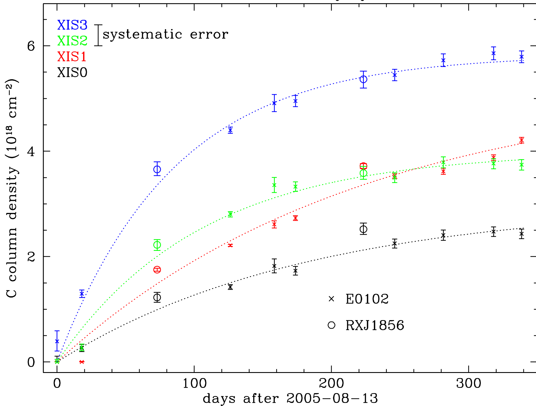
Suzaku/XIS contamination history, N_c/N_0 = 6 assumed, rev0.7
