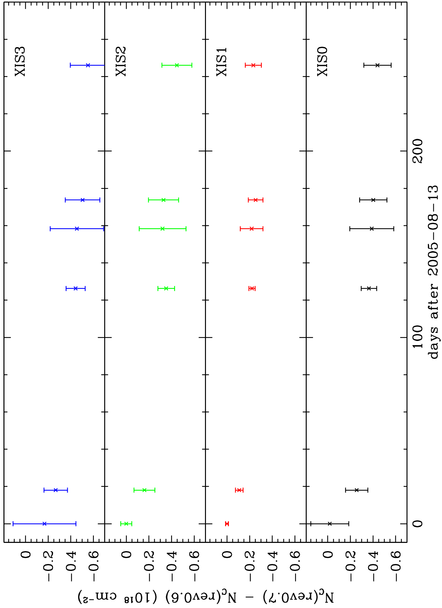
E0102 contamination - rev0.6 vs. rev0.7 comparison (C/O=6)
